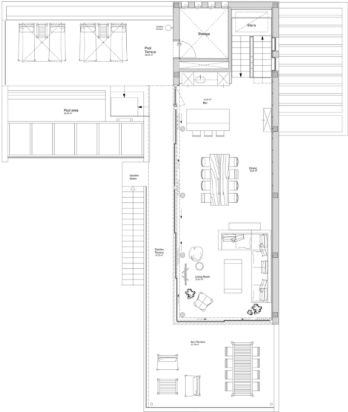
Floor Plan
